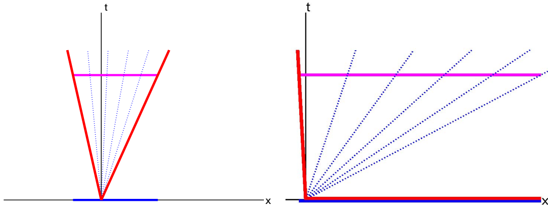
Figure 2.1: Closed conic hulls of two closed convex sets shown in blue : segment (left) and ray (right). Magenta sets are liftings of the blue ones; red angles are the closed conic hulls of blue sets. To get from closed conic hulls the conic hulls per se , you should eliminate from the red angles their parts on the x -axis. When the original set is bounded (left picture), all you need to eliminate is the origin; when it is unbounded (right picture), you need to eliminate much more.
