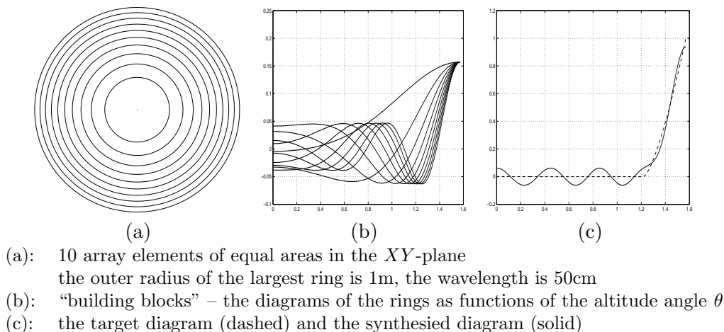
Figure 2.2: Synthesis of antennae array
