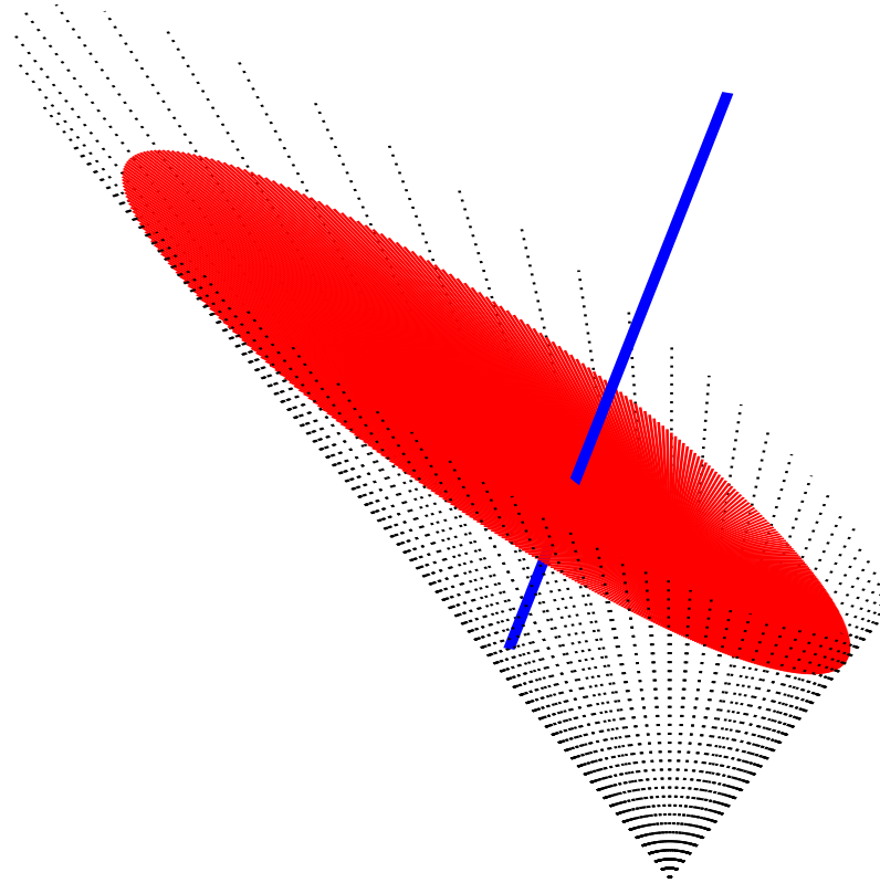
Figure 1.1. Primal-dual pair of conic problems on 3D Lorentz cone Red: feasible set of (P) Blue: feasible set of (D)
