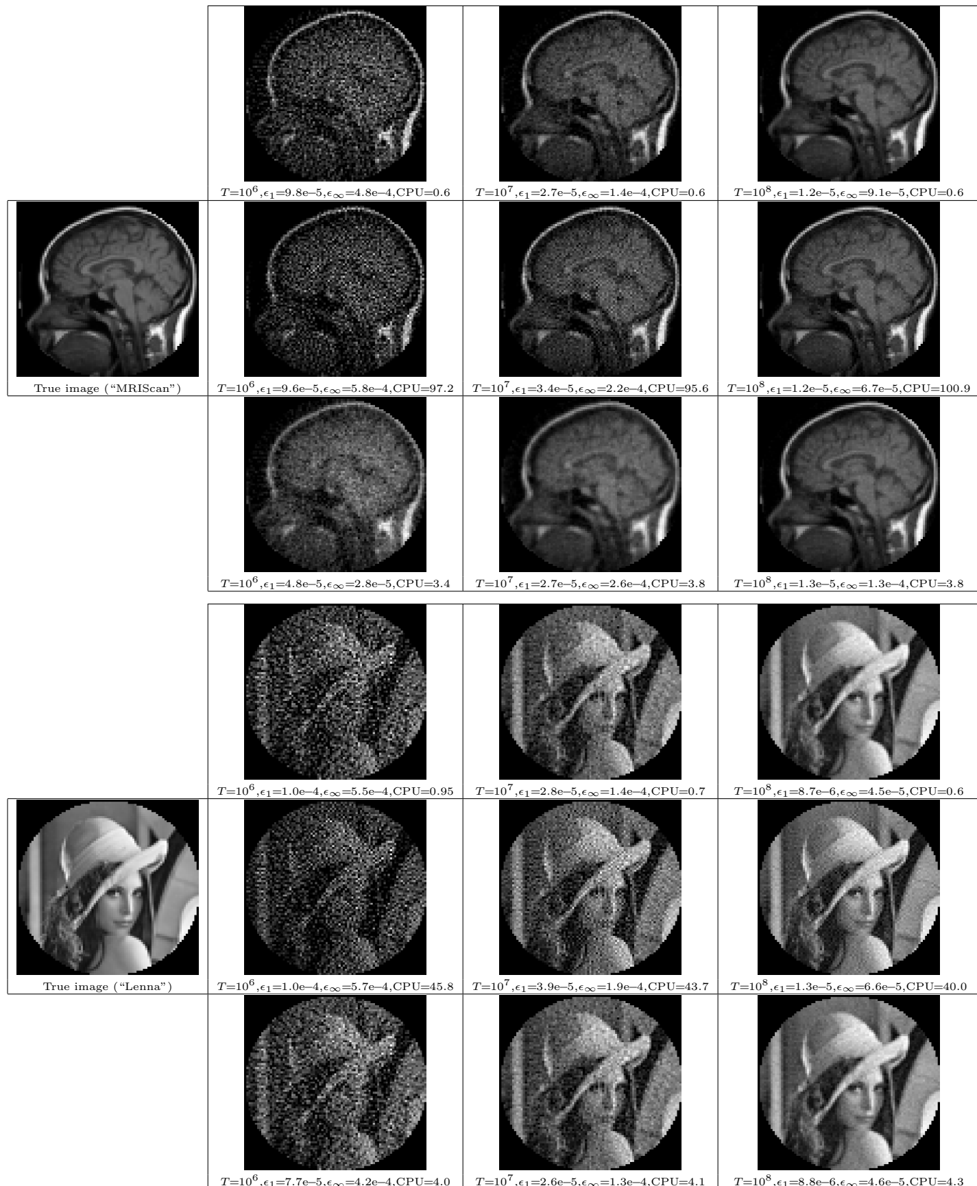
Figure 5.8: PET recovery via Maximum Likelihood and Krylov subspaces, n = 5,664 pixels and m = 18,336 bins. For both images, top, middle, and bottom rows correspond to Krylov Least Squares, Maximum Likelihood, and Krylov Maximum Likelihood recoveries, respectively. CPU is in seconds
